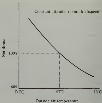
FIGURE 1-74. Effect of OAT on thrust output.
